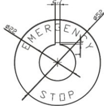
ST-22B
