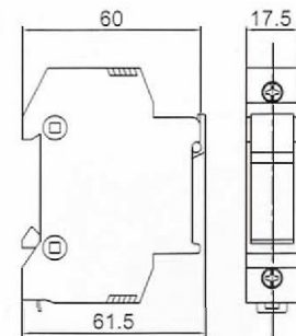
RT18-32 Rail type Fuse holder
