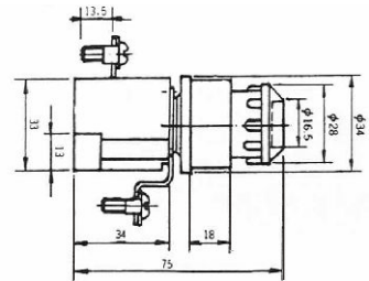
RT18-32 Rail type Fuse holder
